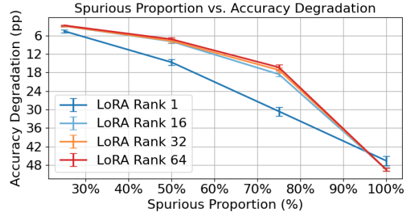
(b) Difference in balanced accuracy ( \downarrow ) between spurious and clean evaluation sets across LoRA ranks on the snowflake-arctic-embed-xs model. 5% of original token amount SSTI. Regardless, SSTI hijacks the model and leads to accuracy degradation.
