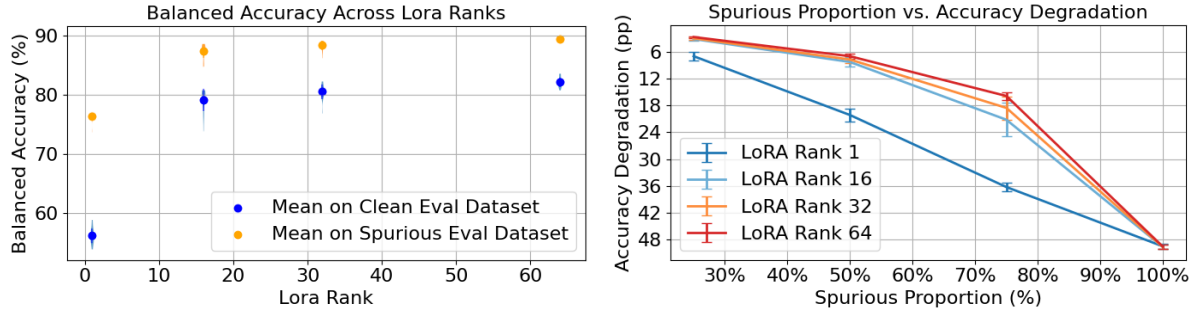
Figure 8.2: Balanced accuracy under Aggressive SSTI (Snowflake-arctic-embed-xs on IMDB) We plot model performance on clean vs. spurious evaluation sets as a function of LoRA rank, under Aggressive SSTI (10% of tokens injected in 50% of training samples). Error bars reflect variation across injection locations and random seeds. (Left) : Balanced accuracy ( \uparrow ) for clean and spurious test sets as a function of LoRA rank. Higher ranks improve alignment between clean and spurious performance—indicating partial recovery from shortcut reliance. (Right) : Accuracy degradation (spurious minus clean) ( \downarrow ) across LoRA ranks. The performance gap shrinks with rank, showing that higher-capacity adapters mitigate spurious reliance under aggressive SSTI.
