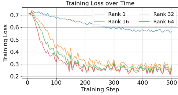
(a) Training loss throughout training across LoRA ranks for Snowflake-arctic-embed-xs on IMDB with aggressive date SSTI.
