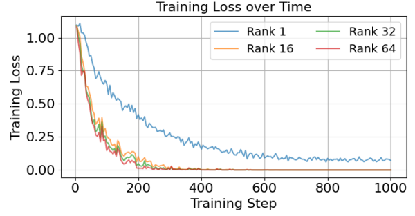
(b) Training loss throughout training across LoRA ranks for Llama-3-8B on Financial Classification with aggressive date SSTI.
