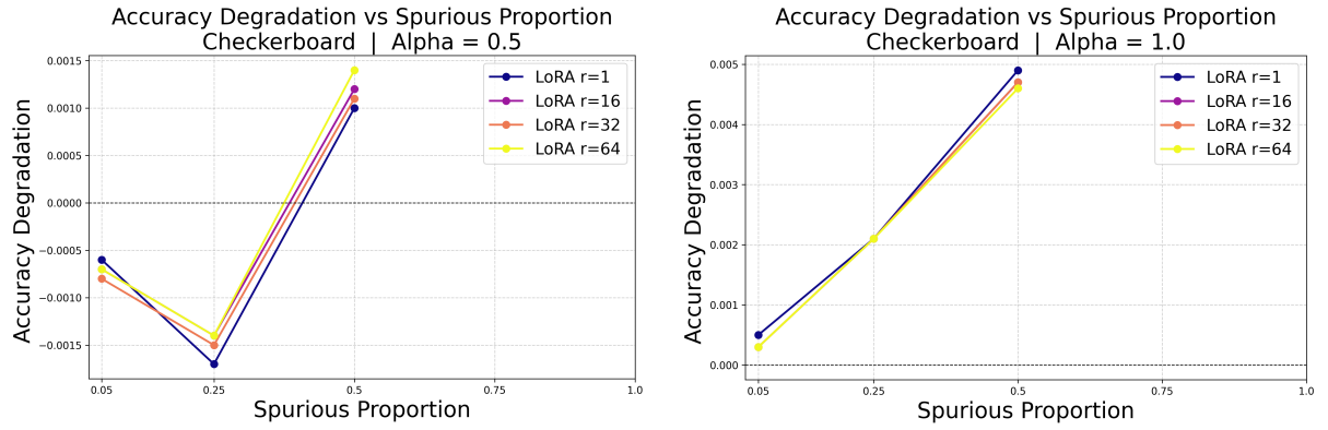
Figure 8.12: Accuracy Degradation across LoRA rank for CLIP (ViT-B/32) on CIFAR10 using a checkerboard SSTI transformation with strength (Left) of 0.5 and (Right) of 1.0. The checkerboard SSTI transformation does not affect Accuracy Degradation.
