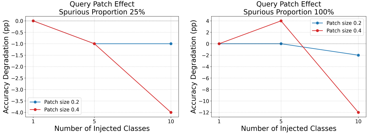
Figure 5.4: Accuracy Degradation(spurious context and spurious query minus spurious context and clean query) for (Left) spurious proportion of 25% and (Right) spurious proportion of 100%. Being exposed to spurious context does not help the model learn shortcut solutions that it can leverage during inference. In fact, it harms performance. Additional results for other spurious proportions can be found in fig. 8.14. Results shown are for Phi-3.5-vision-instruct on CIFAR10 .
