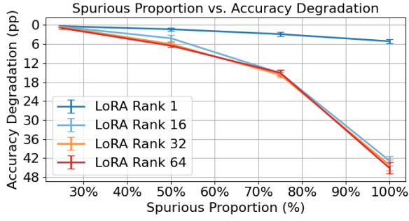
(a) Difference in balanced accuracy ( \uparrow ) between spurious and clean evaluation sets across LoRA ranks on the snowflake-arctic-embed-xs model. Single token SSTI. Regardless, SSTI hijacks the model and leads to accuracy degradation.
