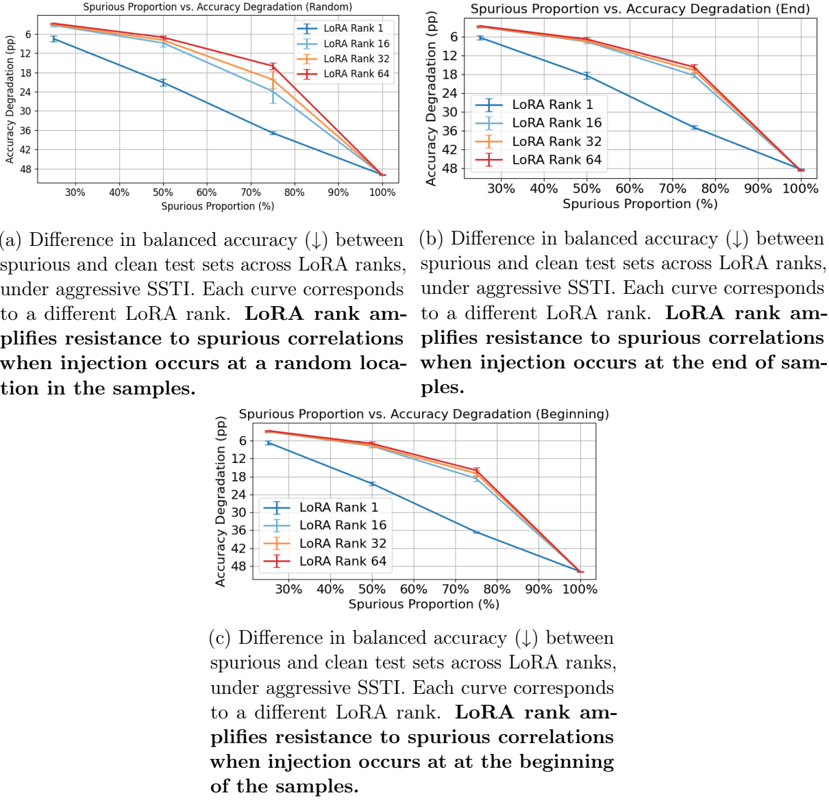
Figure 8.8: Trends hold across different SSTI injection locations: random, beginning, end. ( snowflake-arctic-embed-xs on IMDB )
