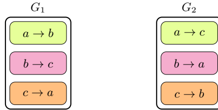
Fig. 3: G_1 : directed triangle in the “forward” direction; G_2 : directed triangle in the “backward” direction. The corresponding MC is not irreducible.
