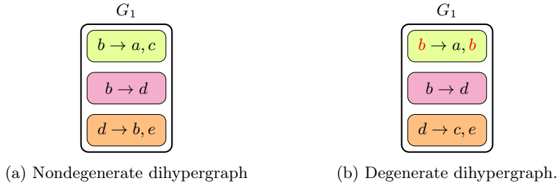
Fig. 1: Examples of dihypergraphs
