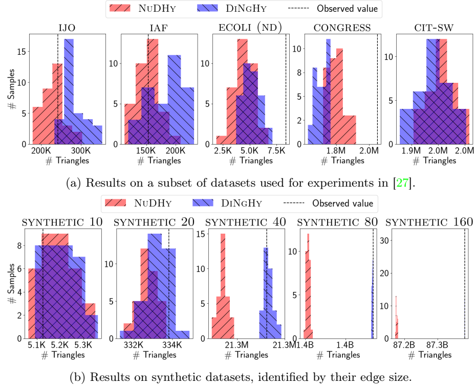
Fig. 8: Empirical distributions of the number of 3-cycles in 33 samples. The observed value is omitted when far from both empirical distributions.
