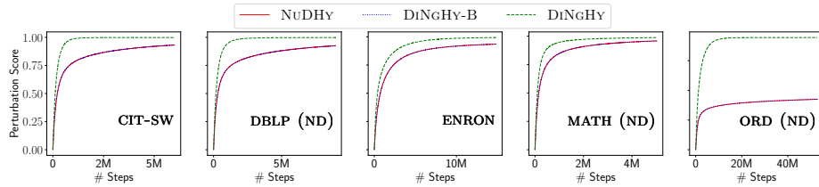
Fig. 9: Perturbation score as function of the steps on the Markov chain. In each case, the curves for NuDHY and DiNGHY-B perfectly overlap.
