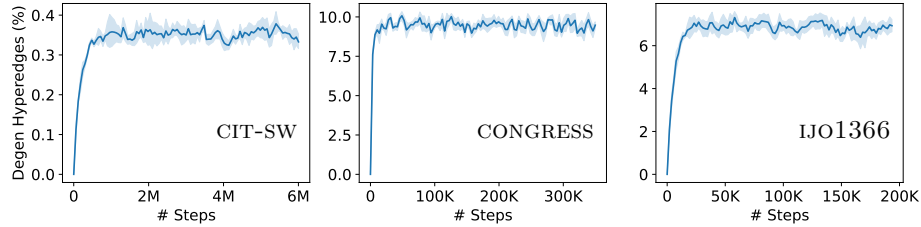
Fig. 7: Mean percentage (over 33 samples, 95% confidence interval shaded) of degenerate hyperdegdes as function of the number of steps of the Markov chain.
