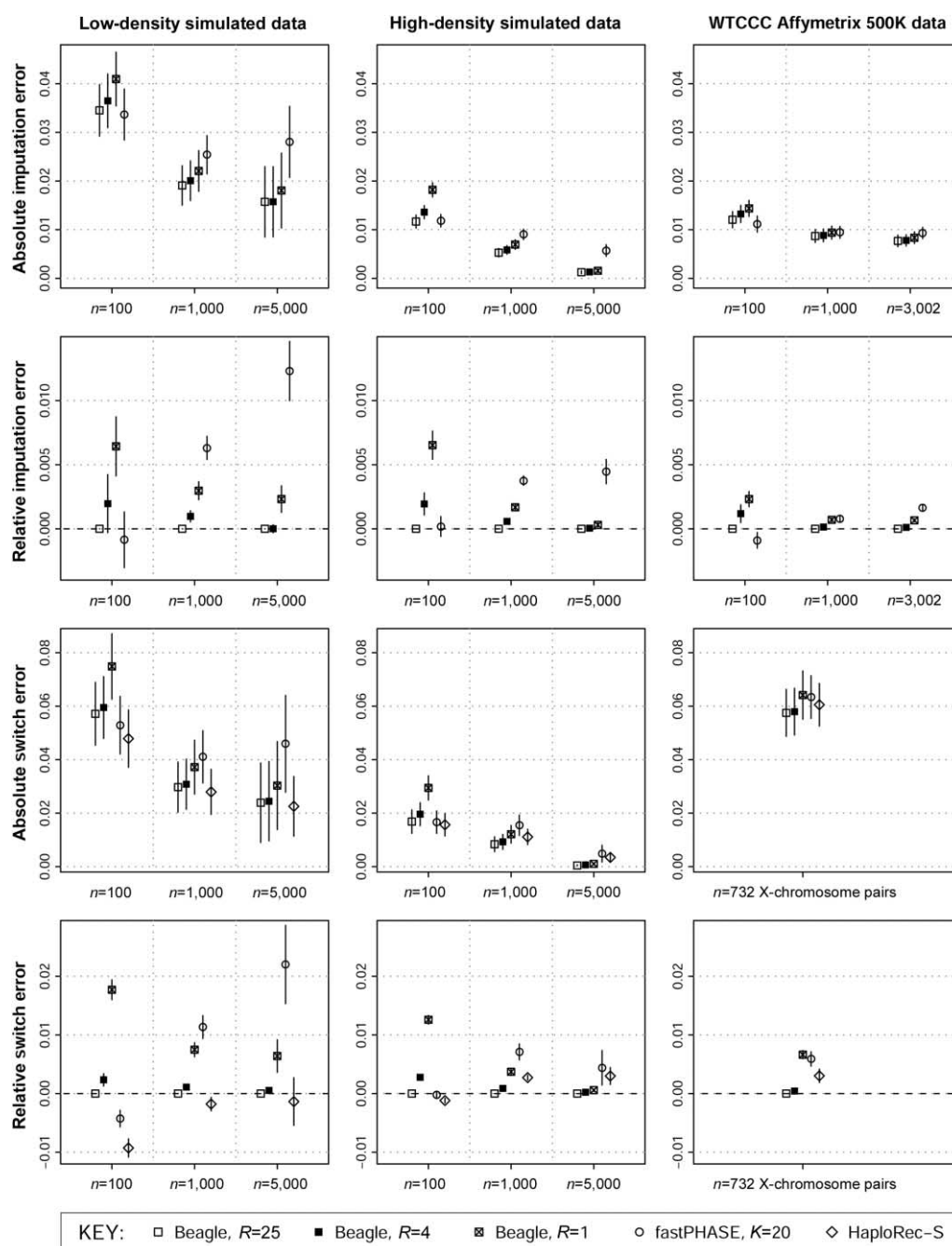
Figure 2. Error rates for selected haplotype-phasing methods. Three classes of data were considered: low-density data with \sim 1 SNP per 10 kb (left column), high-density data with \sim 1 SNP per 3 kb (middle column), and Affymetrix 500K data for the WTCCC controls (right column). Within each plot, three sample sizes ( n ) are shown. Each row of graphs gives a different measure of accuracy (Y-axis). The relative error graphs show differences in error rate between each method and a reference method, which is Beagle with R = 25 samples per individual. All estimates are averaged across the data sets, with error bars showing \pm 2 SEs.
