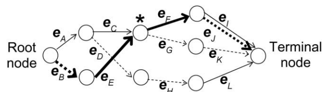
Figure 1. Example of a directed acyclic graph representing the localized haplotype-cluster model for four markers, with the haplotype counts given in table 1. For each marker, allele 1 is represented by a solid line, and allele 2 by a dashed line. The bold-line edges from the root node to the terminal node represent the haplotype 2112. The node marked by an asterisk (*) is the parent node for edge e_F .
