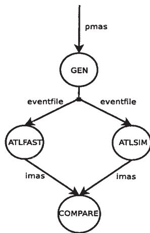
Figure 1: The simplified Atlas Workflow
