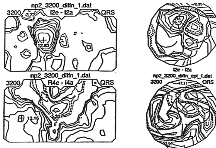
Figure 9: Body surface (left) and epicardial surface (right) potential difference maps for the same patient during PTCA. Upper maps from an occlusion of the left anterior descending artery; lower maps from occlusion of the right coronary artery.
