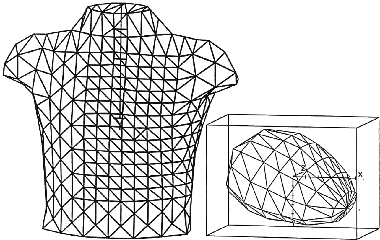
Figure 8. Dalhousie torso (left) and epicardium (right).
