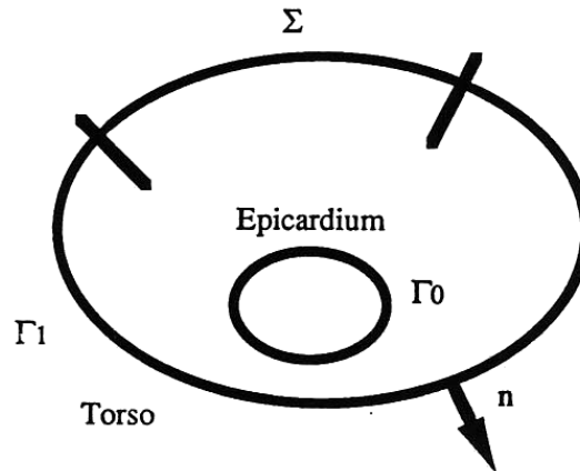
Figure 1. Geometry for the electrocardiographic field equation.
