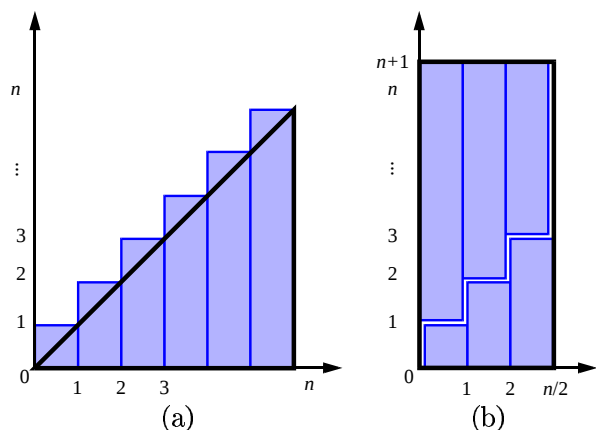
Figure 1: Visual justifications of Proposition 2.1. Both illustrations visualize the identity in terms of the total area covered by n unit-width rectangles with heights 1, 2, \dots, n . In (a) the rectangles are shown to cover a big triangle of area n^2/2 (base n and height n ) plus n small triangles of area 1/2 each (base 1 and height 1 ). In (b), which applies only when n is even, the rectangles are shown to cover a big rectangle of base n/2 and height n+1 .
