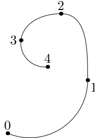
Figure 6: The result of draw z0..z1{up}..z2{left}..z3..z4 .
