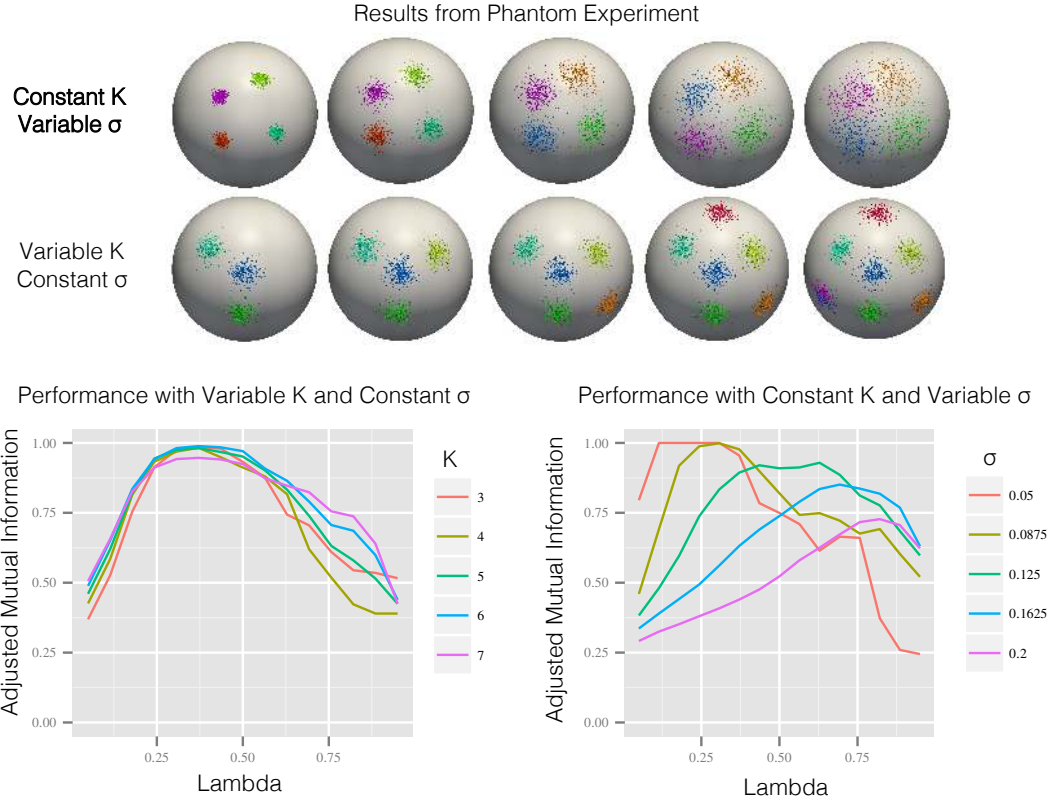
Figure 3.1: Results from the first experiment described in Sec. 3.4.1, showing visualizations of the synthetic axial data and the optimal clusterings computed from the proposed method. The top shows results for variable cluster size \sigma = \{0.05, 0.0875, 0.125, 0.1625, 0.2\} , and constant number of clusters N = 4 . The bottom shows results for constant cluster size \sigma = 0.10 , and variable number of clusters N = \{3, 4, 5, 6, 7\} . The bottom right shows a single mislabeled cluster, possibly caused by finding a local minima in the optimization. First experiment: clustering performance as a function of cluster penalty parameter \lambda \in [0, 1] given ground truth generated with cluster size \sigma , and number of clusters N . We measured the adjusted mutual information (AMI), a statistical measure takes a maximal value when clusterings are equivalent. Shown are plots of the AMI vs. \lambda for two conditions. The first tested with variable \sigma = \{0.05, 0.0875, 0.125, 0.1625, 0.2\} and constant N = 4 . The second tested with constant \sigma = 0.10 and variable N = \{3, 4, 5, 6, 7\} . These results indicate that the optimal \lambda depends more on \sigma than N , suggesting that performance may depend on the noise level and may diminish when differing clusters sizes are present. Also note that the maximum AMI decreases with increasing \sigma , which may be due to cluster overlap or over-sensitivity in the AMI measure.
