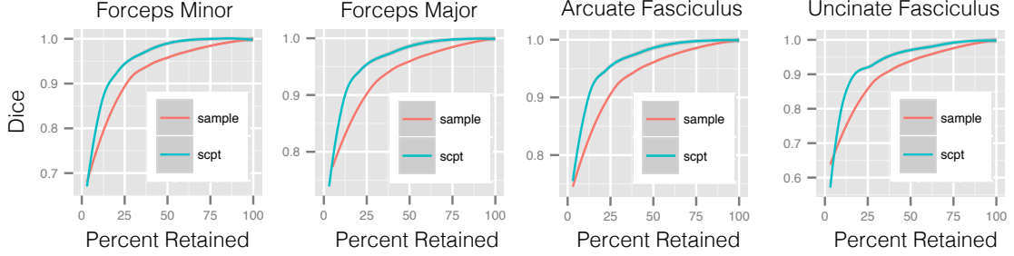
Figure 5.4: Results from the third experiment described in Sec. 5.3.5. This shows performance of the simplification algorithm in several bundles. Each plot shows the simplification error measured with the Dice coefficient. The proposed method was compared to random sampling, and both methods are plotted by the percentage of curves retained from simplification. The results show the proposed method performs consistently better in nearly all cases.
