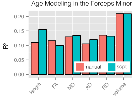
Figure 5.6: Results from the fifth experiment described in Sec. 5.3.7 testing the sensitivity to normal aging in a population of 80 subjects. The analysis focused on the forceps minor, which traverses the anterior portion of the corpus callosum and has well documented changes with age. The proposed population-based analysis was compared to a manual region-based approach in six fiber bundle metrics: fractional anisotropy (FA), mean diffusivity (MD), radial diffusivity (RD), axial diffusivity, bundle length, and bundle volume. For each bundle measure and method, multiple linear regression models were fit to model age with respect to intracranial volume, sex and each tractography-based metric. The plot shows the resulting R^2 of each model (bigger is better), showing comparable performance in bundle volume, MD, and RD, improved performance in bundle length, and AD, and slightly worse performance in FA.
