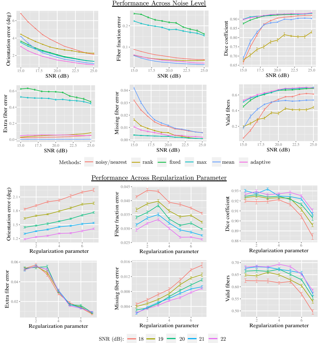
Figure 6.8: Results from the second experiment in Sec. 6.4.3 using the phantom shown in Fig. 6.6. Evaluation was first performed by measuring voxel-wise orientation error, volume fraction error, missing fiber error, extra fiber error (lower is better). Tractography-based evaluation was performed to evaluate performance in connectivity mapping using the Dice coefficient and fraction of valid connections (higher is better). Several methods for model selection were compared included: fixed count, local-max selection, mean selection, and our proposed adaptive selection. We also included rank-based estimation and nearest neighbor interpolation to serve as a baseline. The top two rows show performance across noise levels from SNR 15 to 25. We see that adaptive estimation provided significantly lower orientation error than other methods. Across all noise levels, fixed and local-max selection introduced a high volume fraction error and extra fiber error, due to “fiber-splitting”. Adaptive performance significantly reduced these errors with a slight increase in missing fiber error. We also varied the regularization parameter and plotted with semilog axes, x = \log_{10}(1 - \lambda) . We found performance to be acceptable between \lambda = 0.99 and 0.9999 , with a tradeoff between extra and missing fiber error.
