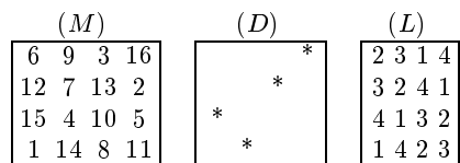
Fig. 2. Structure of solutions: Square M shows a typical diagonally ordered magic square of order 4. In D , we can see how the n largest numbers are distributed very nicely over the square. By associating symbol 1 with numbers 1, \dots, 4 , symbol 2 with numbers 5, \dots, 8 , symbol 3 with numbers 9, \dots, 12 and finally symbol 4 with numbers 13, \dots, 16 , we get the square L . We observe: L is a Latin square!
