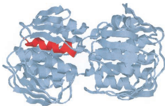
Fig. 4. A ribbon diagram of the structure of UDP-N-acetylglucosamine enolpyruvyl transferase as reported by Skarzynski et al. (1996). The 12 consecutive hydrophobic residues at positions 24–35 are highlighted. The image was prepared with RasMol version 2.6.
