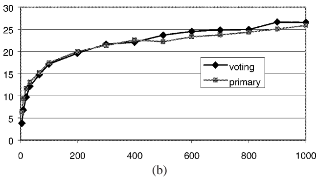
Figure 4. Commit rates: (a) shows the average number of intervals needed for the first replica to commit an update versus the number of replicas for the default voting scheme, voting assuming reliable communication, and a primary-copy scheme; (b) shows the number of intervals for last replica to commit updates.
