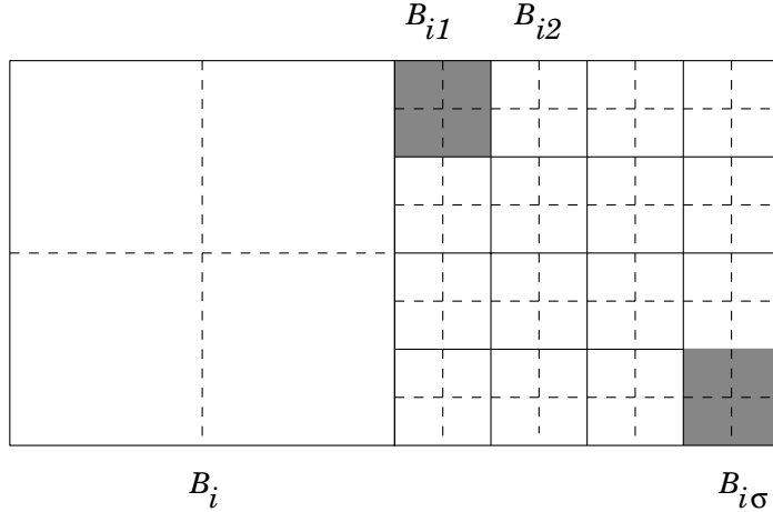
Fig. 4. The box on the left shows large grid and the one on the right shows small grid as well as the subboxes. In this figure, \alpha = 4 and \sigma = 16 .
