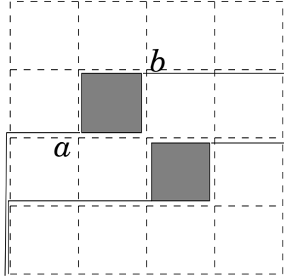
Fig. 5. The lower bound construction showing \rho(\mathcal{F}) = \Omega(\alpha) .
