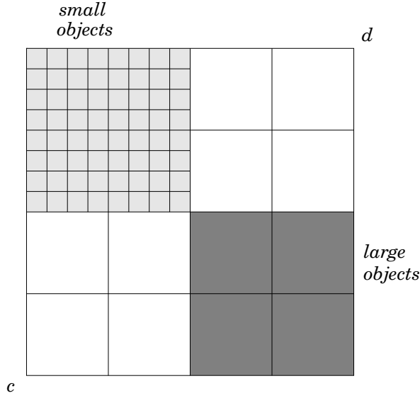
Fig. 6. The lower bound construction, showing \rho(\mathcal{F}) = \Omega(\alpha\sqrt{\sigma}) .
