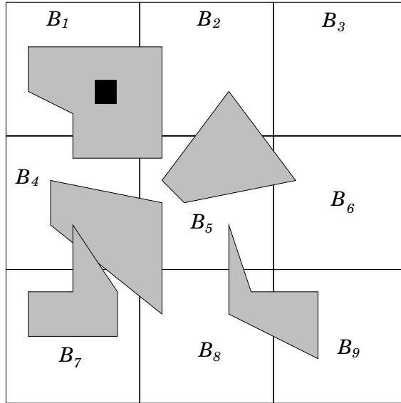
Fig. 2. Tiling of the plane by boxes of size \alpha . The unit size core for the object in B_1 is also shown.
