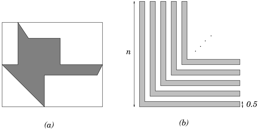
Fig. 1. (a) A polygonal object and its axis-aligned bounding box. (b) An example with K_b = \Omega(n^2) and K_o = O(1) .
