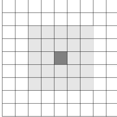
Fig. 3. A box, shown in dark at the center, and its 24 neighbors.
