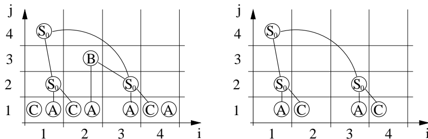
Figure 2: We show how the algorithm works when the initial domain of X_3 is D_3 = \{\{\}\} . The left picture shows sets S_{ij} and the right the sets S'_{ij} . We see that the constraint filtering algorithm determines the only word in L_G \cap D_1 \dots D_4 is “ \{\}\{\} ”.
