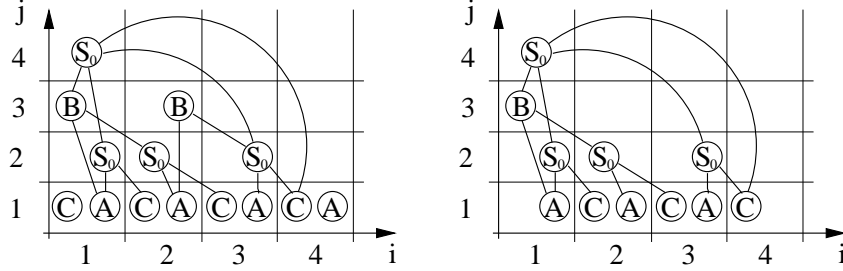
Figure 1: Context-Free Filtering: A rectangle with coordinates (i, j) contains nodes v_{ijA} for each non-terminal A in the set S_{ij} . All arcs are considered to be directed from top to bottom. The left picture shows the situation after step (2). S_0 is in S_{14} , therefore the constraint is satisfiable. The right picture illustrates the shrunken graph with sets S'_{ij} after all parts have been removed that cannot be reached from node v_{14S_0} . We see that the value ']' will be removed from D_1 and '[' from D_4 .
