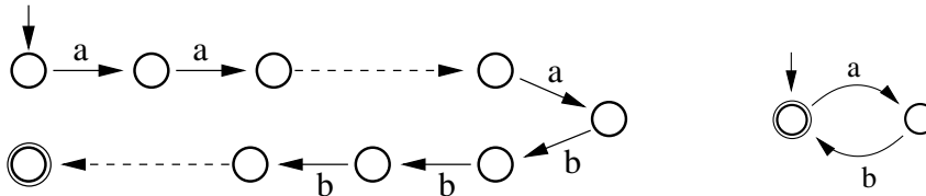
Figure 3: Regular grammar filtering for \{a^n b^n\} . The left figure shows a linear-size automaton, the right an automaton that accepts a reordering of the language.
