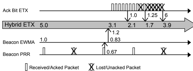
Figure 5: Our link estimator combines estimates of ETX separately for unicast and broadcast traffic with window sizes of k_u = 5 and k_b = 2 respectively. The latter are first themselves averaged before being combined. We show incoming packets are light boxes, marking dropped packets with an “X”. The estimator calculates link estimates for each of the two estimators at the times indicated with vertical arrows.
