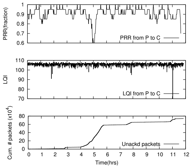
Figure 3: Unaware of the reduced PRR, MultiHopLQI attempts to deliver packets on the same link between the fourth and sixth hour causing increased number of retransmissions due to unacknowledged packets.
