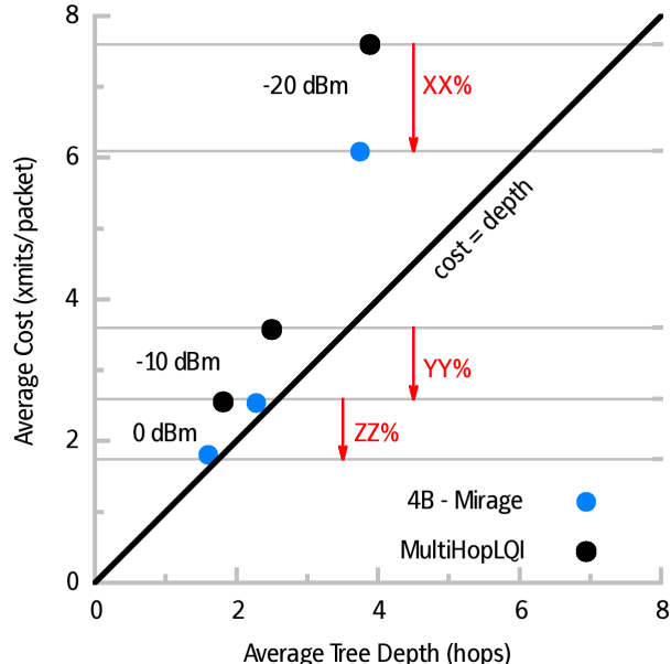
Figure 7: Average node depth and cost for MultiHopLQI and 4B for decreasing transmit powers on the Mirage testbed. 4B reduces cost by 19-28%.
