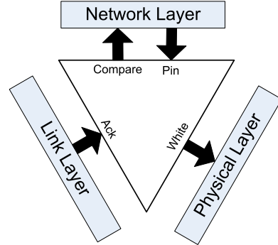
Figure 4: A link estimator, represented by the triangle in the center, uses four bits of information from the three layers. Outgoing arrows represent information the estimator requests on packets it receives. Incoming arrows represent information the layers actively provide.
