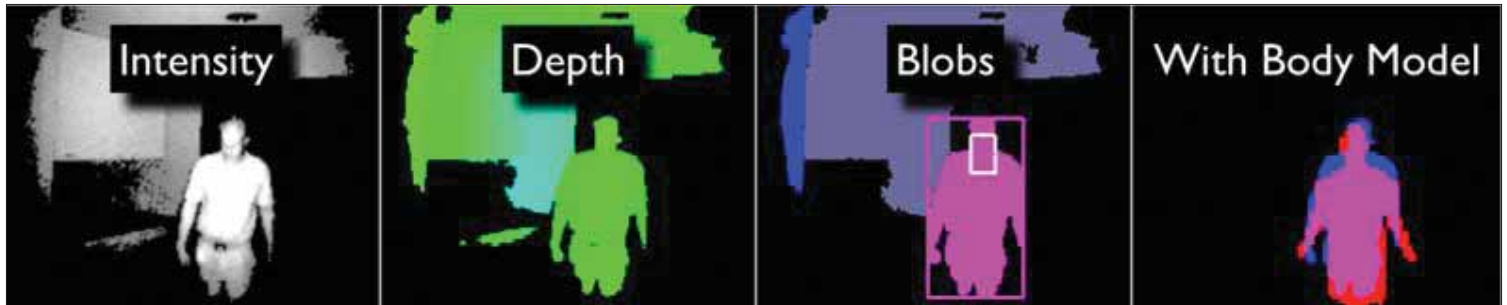
An illustration of our perception pipeline.
