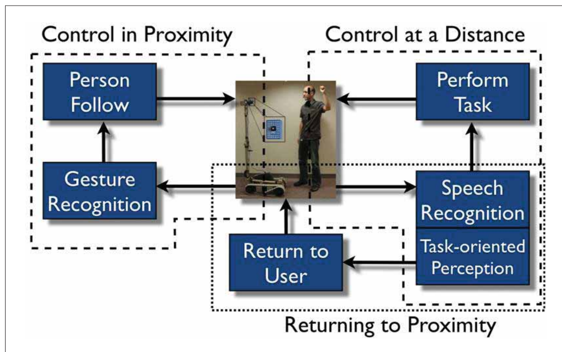
An illustration of the relationship between interaction modalities and human-robot distance in our framework.
